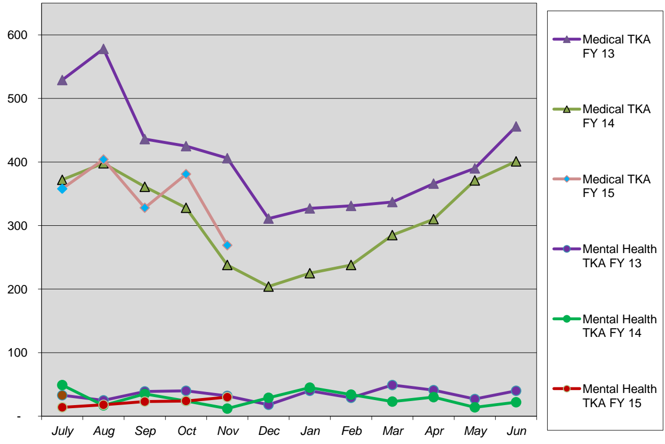
Talkeetna Encounter History
