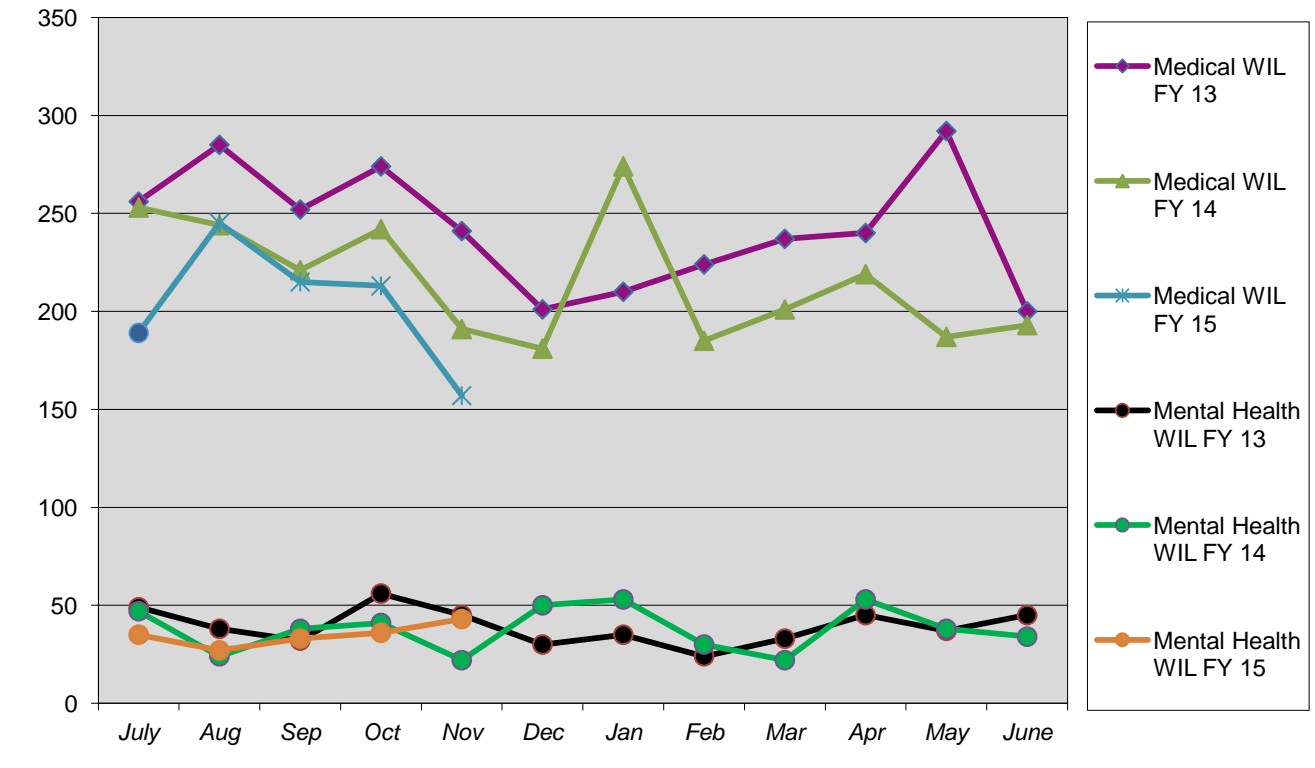
Willow Encounter History
